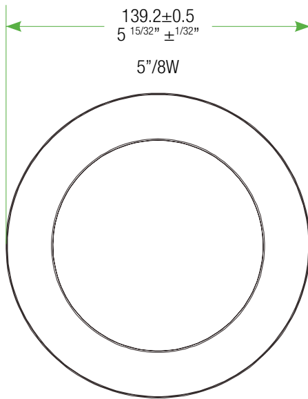
8W Fixture
