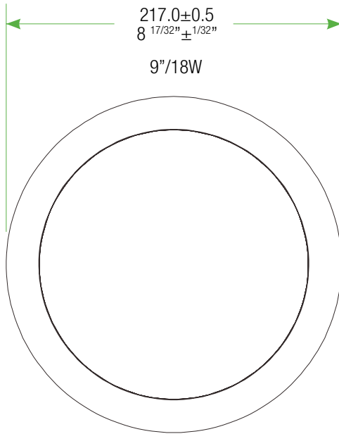
18W Fixture
