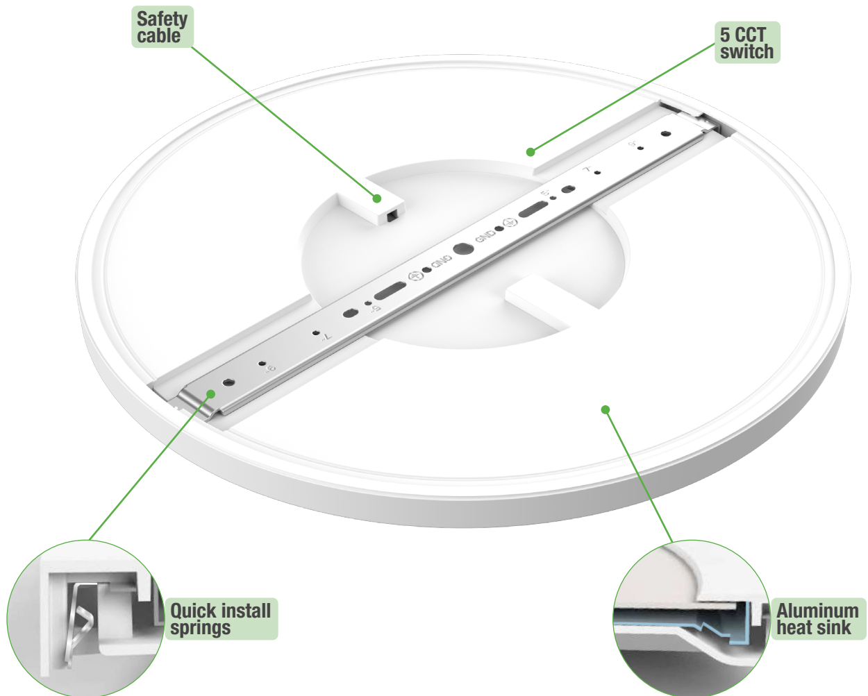
JB Installation
