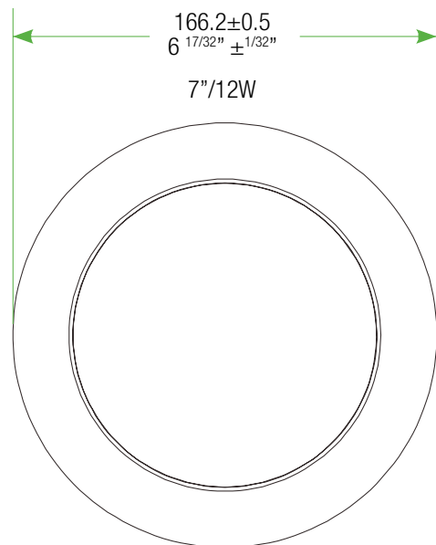
12W Trim ring
