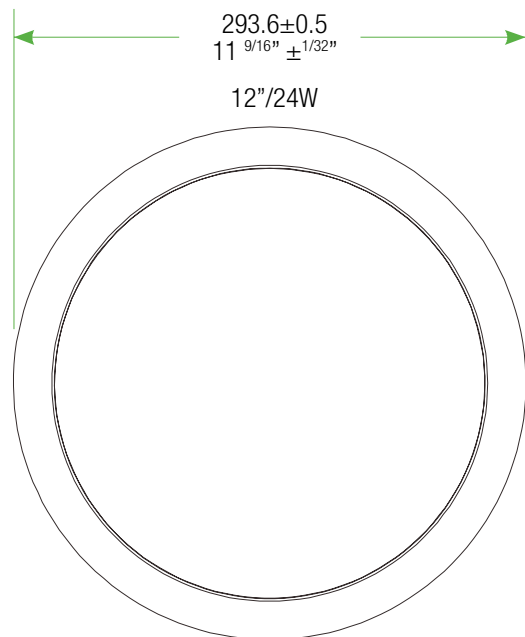
24W Trim ring
