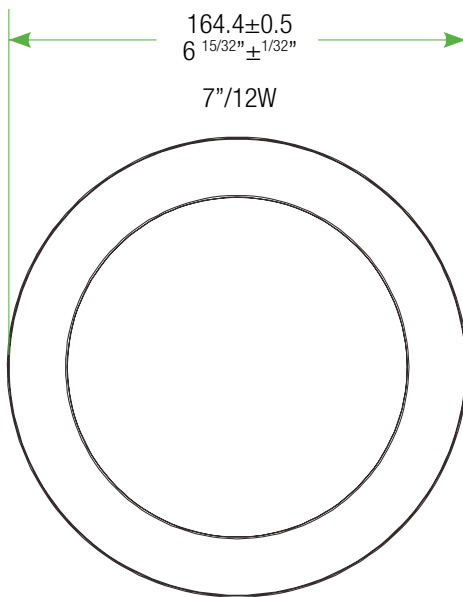
12W Fixture
