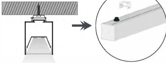
Surface installation
