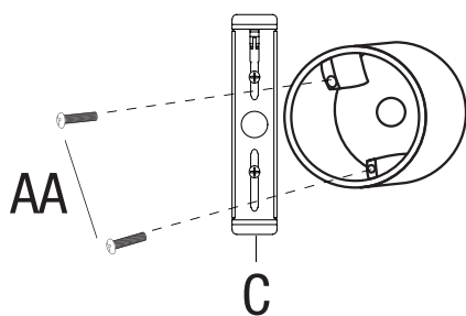
Wall Mount
