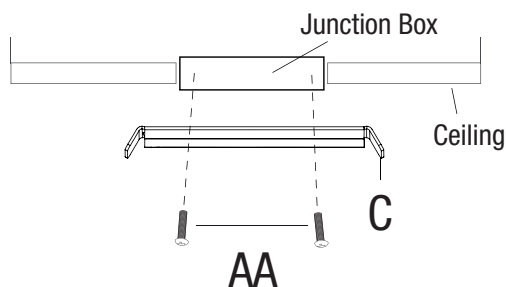
Ceiling Mount
