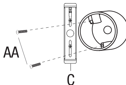
Wall Mount
