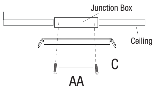
Ceiling Mount
